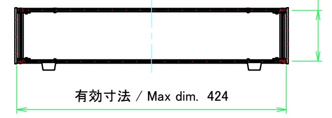
C-C (1:6)
