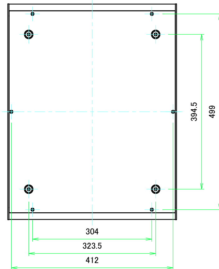
F view
