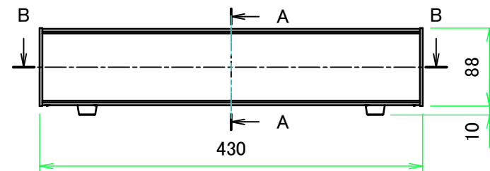
F view
