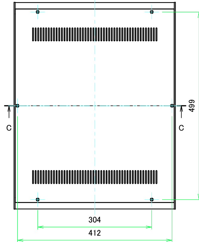
A view
